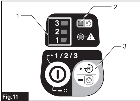
Fig.11 ► 1. Speed indicator 2. ADT indicator 3. Reverse button
